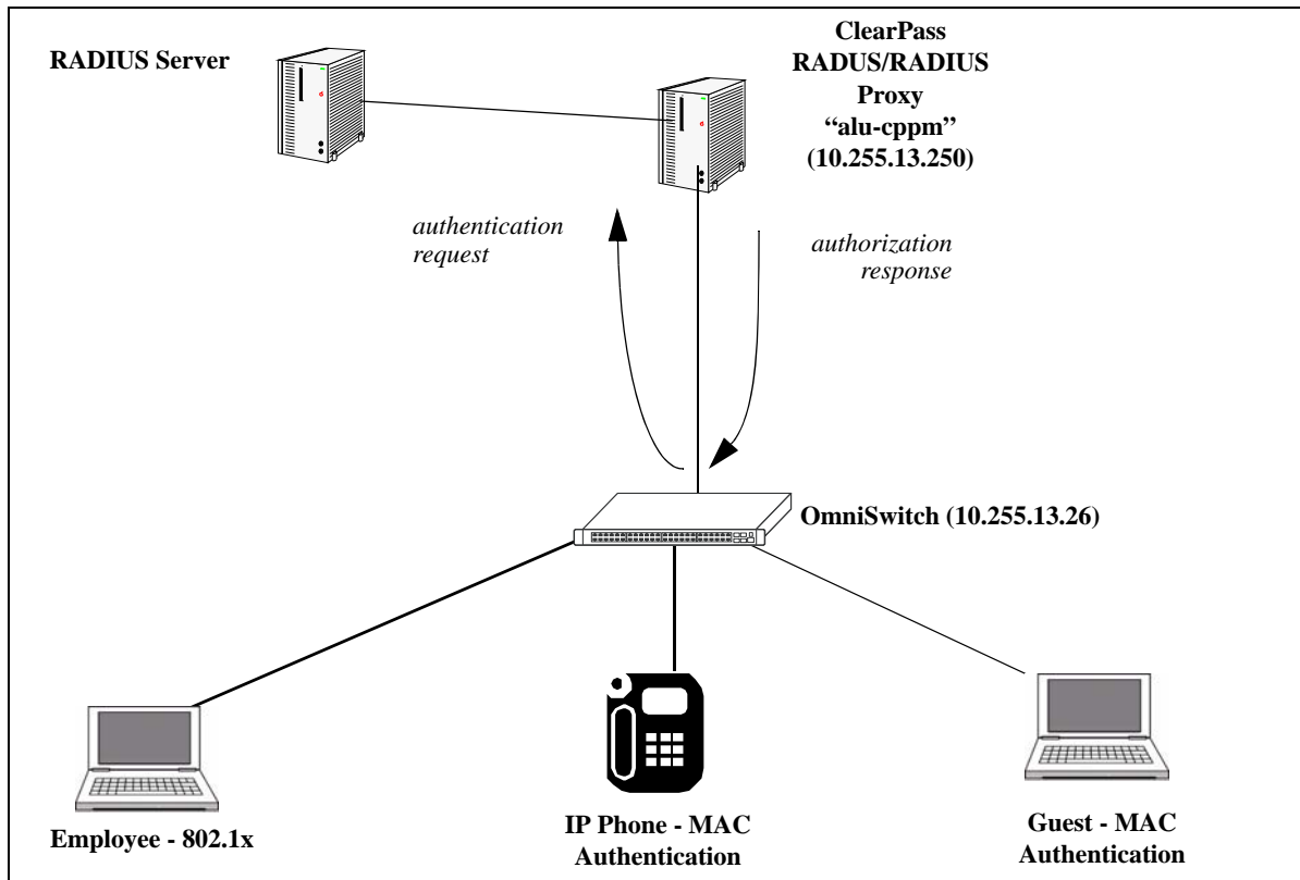
BYOD network with Employee and Guest devices
